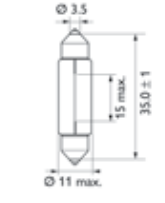
C5W
