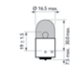
RY10W
