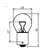
Stop P25
