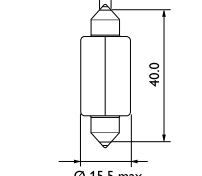
Festoon T15x43
