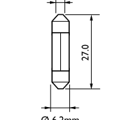
Festoon T6,2x27
