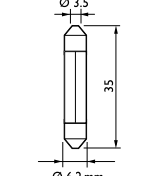
Festoon T6,2x35
