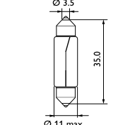
Festoon T10,5x38
