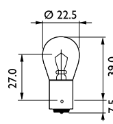
Stop P22
