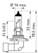
HB4
