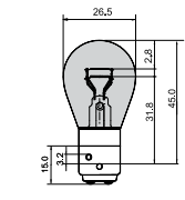
PR21/5W
