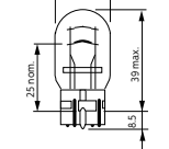
W21/5W
