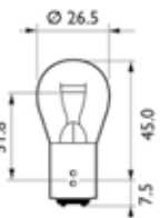
P21/5W
