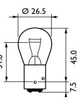
P21/4W
